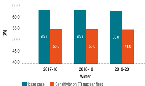
INSTALLED NUCLEAR CAPACITY CONSIDERED IN FRANCE FOR THE 'BASE CASE' AND FOR THE SENSITIVITY ON THE FRENCH NUCLEAR FLEET (FIG. 77)
