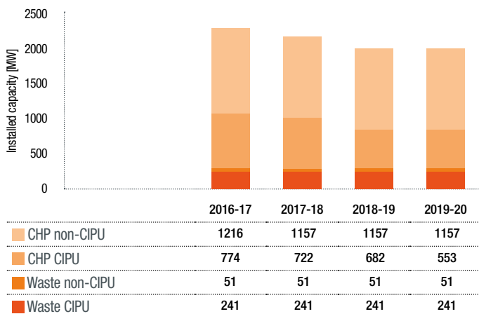
FORECASTED EVOLUTION OF INSTALLED CAPACITY CHP AND WASTE (FIG. 44)
