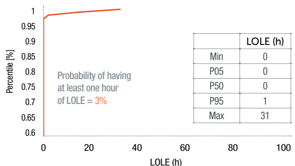
WINTER 2018-19 – 'BASE CASE' CUMULATIVE DISTRIBUTION OF LOLE WITHOUT STRATEGIC RESERVE (FIG. 115)
