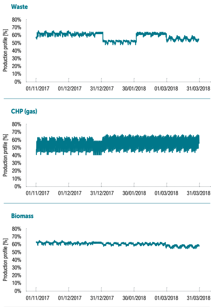
HOURLY AVERAGE PRODUCTION PROFILE FOR THE WINTER (FIG. 47)
