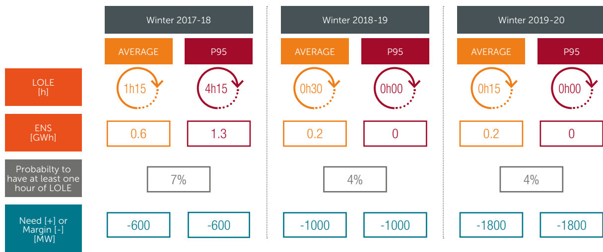
SENSITIVITY TO THE 'LOW' THERMAL GENERATION FACILITIES FOR FRANCE (ASSUMING A 'CARBON TAX' AND NO 'CRM' (FIG. 132)
