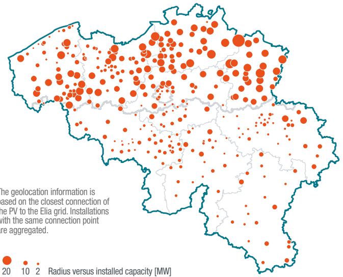
GEOGRAPHICAL DISTRIBUTION OF THE BELGIAN PHOTOVOLTAIC ELECTRICITY PRODUCTION (WINTER 2016-17) (FIG. 41)
