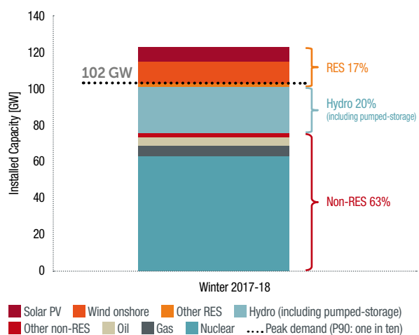
INSTALLED CAPACITY CONSIDERED IN THE 'BASE CASE' AND PEAK DEMAND FOR WINTER 2017-18 IN FRANCE (FIG. 82)
