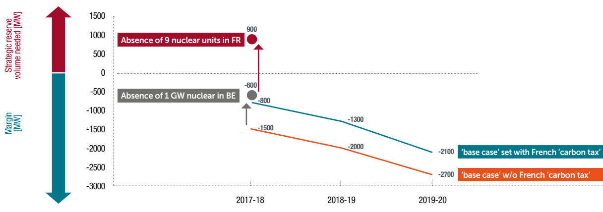
RESULTS FOR 'BASE CASE' WITHOUT FRENCH 'CARBON TAX' AND IMPACT OF THE ABSENCE OF 1 GW BELGIAN AND 9 FRENCH NUCLEAR UNITS DURING THE WHOLE WINTER
