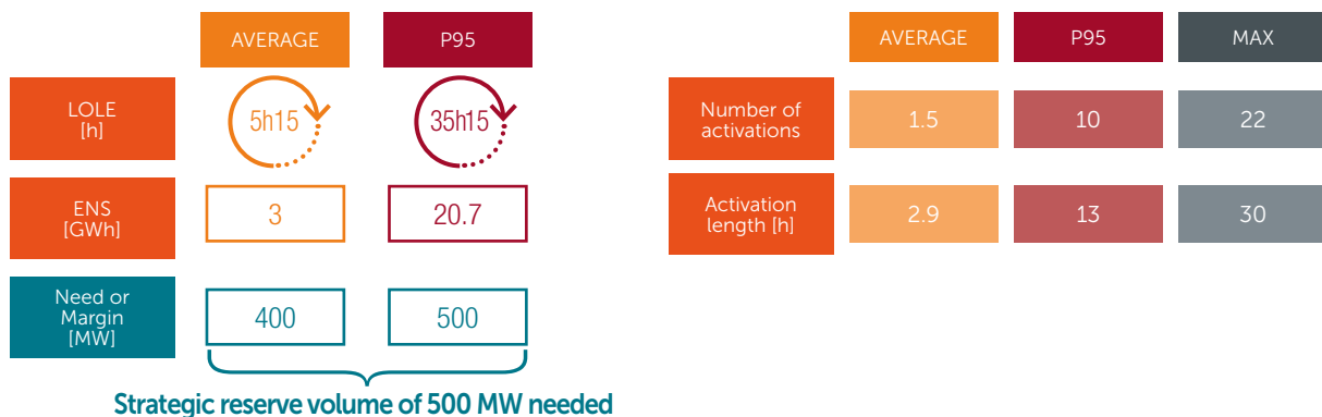
WINTER 2017-18 – SENSITIVITY TO THE FRENCH NUCLEAR FLEET (ABSENCE OF 9 UNITS) (FIG. 134)
