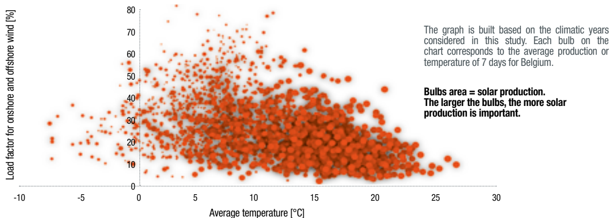
CORRELATION BETWEEN WIND PRODUCTION, SOLAR PRODUCTION AND TEMPERATURE (AVERAGE OF 7 DAYS) (FIG. 14)
