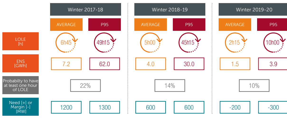
SENSITIVITY TO THE ABSENCE OF 2GW NUCLEAR CAPACITY IN BELGIUM (FIG. 130)
