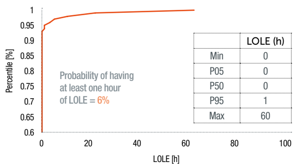
WINTER 2017-18 – 'BASE CASE' CUMULATIVE DISTRIBUTION OF LOLE WITHOUT STRATEGIC RESERVE (FIG. 104)
