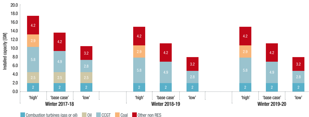
INSTALLED CAPACITY CONSIDERED FOR THE 'BASE CASE', 'LOW' AND 'HIGH' SENSITIVITIES FOR THE FRENCH GENERATION FACILITIES (EXCLUDING NUCLEAR) (FIG. 76)
