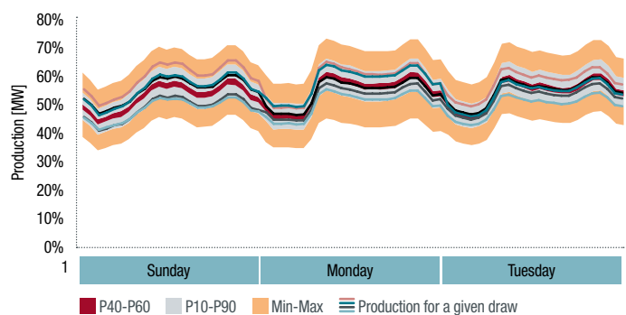
COMBINED CHP, WASTE AND BIOMASS PRODUCTION FOR THE BELGIAN UNITS WITHOUT A CIPU CONTRACT: ILLUSTRATION OF THE DISTRIBUTION FOR A SUNDAY, MONDAY AND TUESDAY (FIG. 48)
