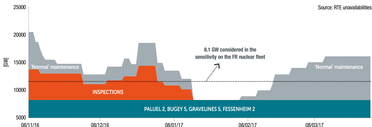
WINTER 2016-17 FRENCH NUCLEAR POWER PLANTS IN MAINTENANCE OR FOR INSPECTIONS (STATUS: 07/11/2016) (FIG. 78)
