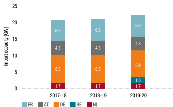
ASSUMPTIONS REGARDING THE MAXIMUM IMPORT CAPACITY ONLY FROM COUNTRIES OUTSIDE THE CWE ZONE (FIG. 102)
