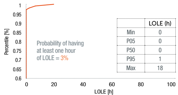
WINTER 2019-20 – 'BASE CASE' CUMULATIVE DISTRIBUTION OF LOLE WITHOUT STRATEGIC RESERVE (FIG. 117)
