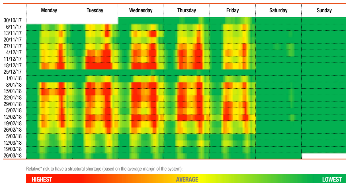
RELATIVE RISK TO HAVE A STRUCTURAL SHORTAGE HOUR FOR WINTER 2017-18 BASED ON THE AVERAGE MARGIN ON THE SYSTEM (FIG. 107)
