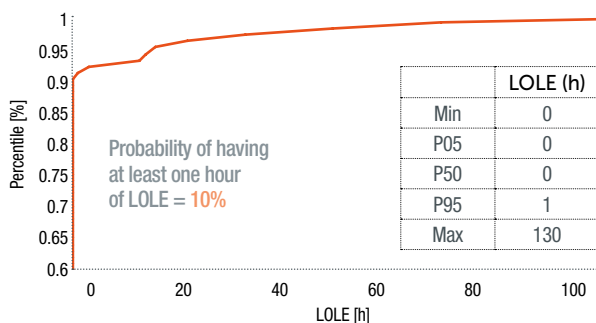
WINTER 2017-18 – SENSITIVITY TO HIGHER FORCED OUTAGE RATES FOR BELGIAN NUCLEAR AND CCGTS: CUMULATIVE DISTRIBUTION OF LOLE WITHOUT STRATEGIC RESERVE (FIG. 127)
