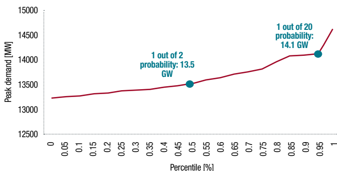
PEAK LOAD DISTRIBUTION FOR THE 40 CLIMATE YEARS FOR BELGIUM FOR THE WINTER 2017-18 (FIG. 69)
